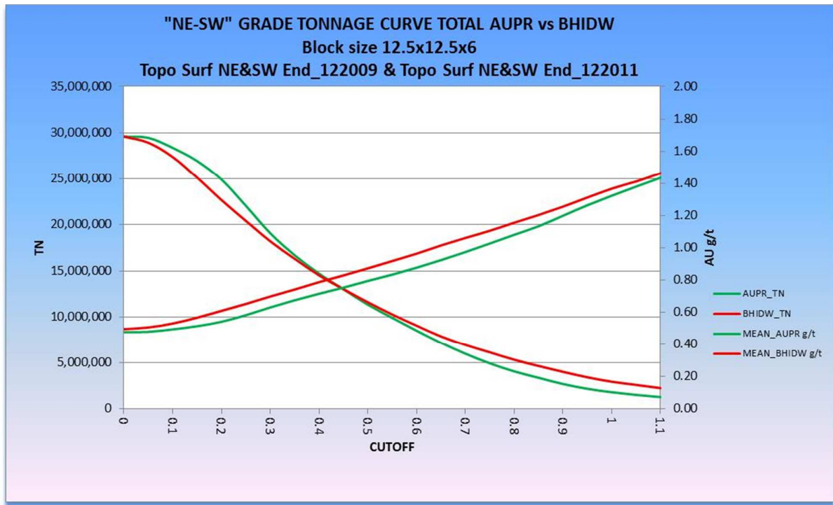
Figure 14-9 Grade Tonnage Curves NE and SW Zones Combined
